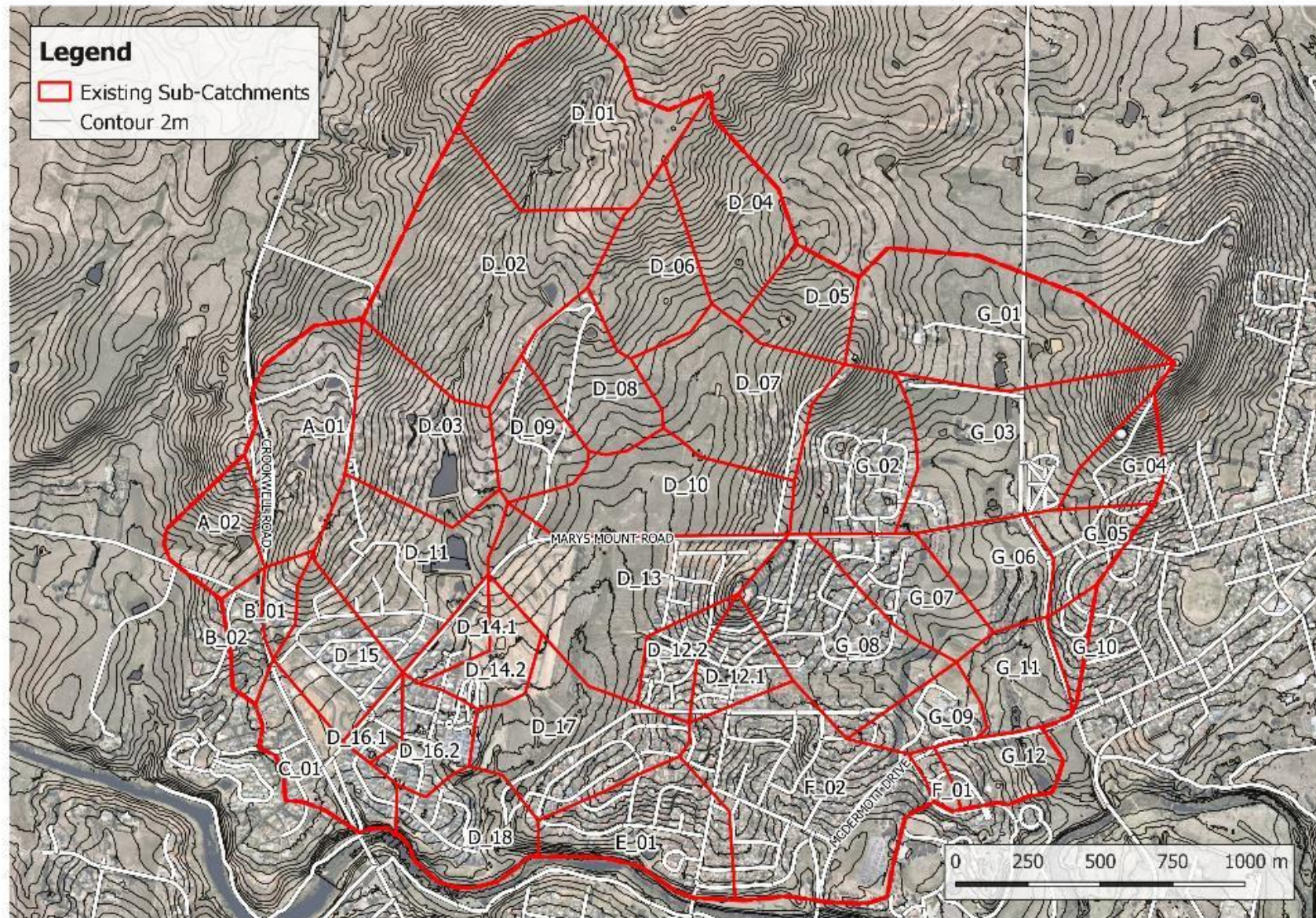
Figure 19-2 Hydrological Catchments (2m Contours)
