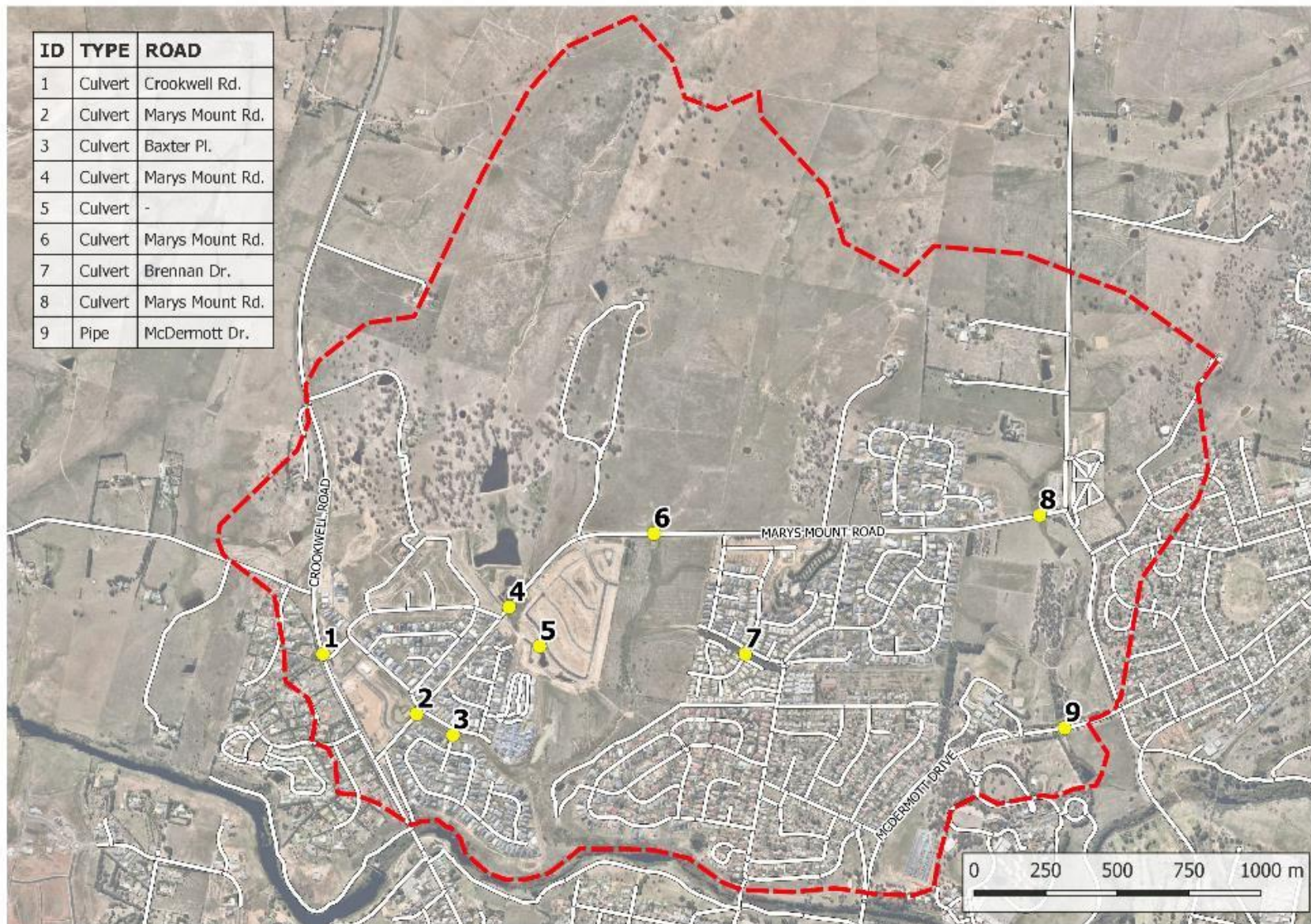
Figure 19-4 Culvert locations
