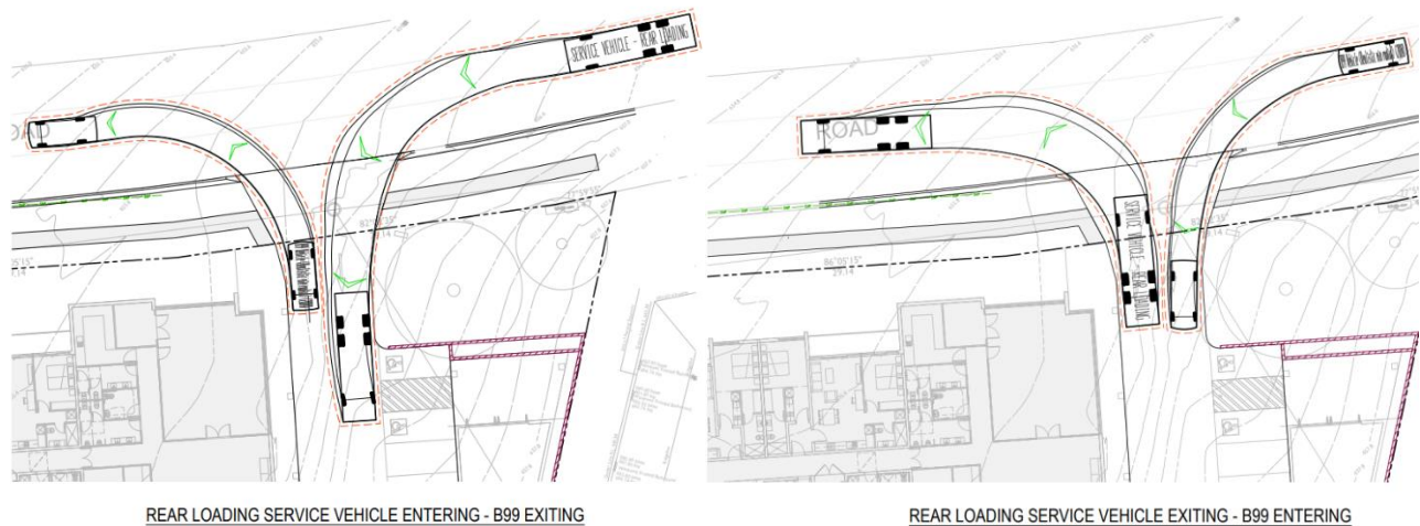
Figure 7 - Service Vehicle Driveway Check
