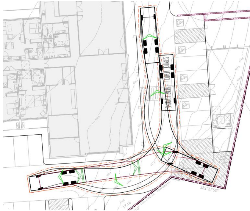
Figure 10 - Service Vehicle Loading Zone Checks
