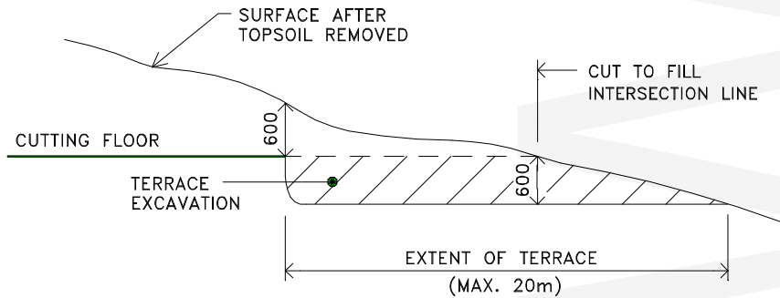
Figure C213.1 - Transition from Cut to Fill
