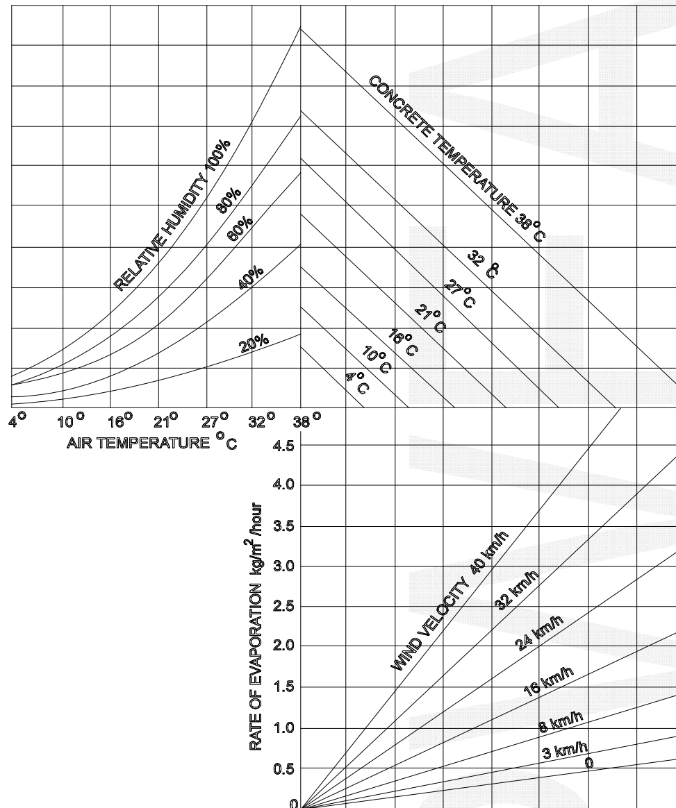
Figure C248.1 - Rate of Evaporation
