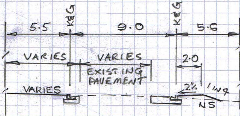
SECTION 'B' LOOKING NORTH.
