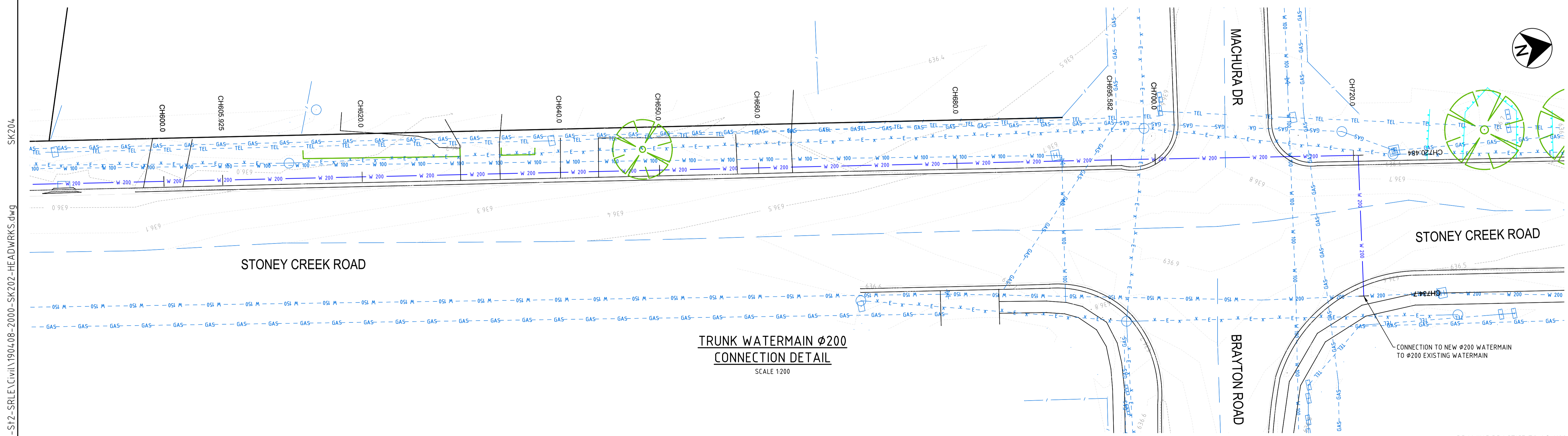
TRUNK WATERMAIN Ø200 SCALE 1:1000
