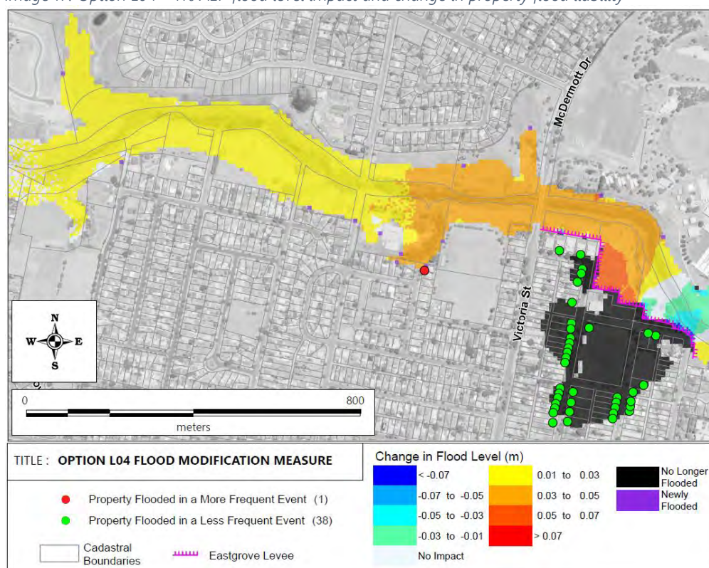
Image 17: Option L04 – 1% AEP flood level impact and change in property flood liability
