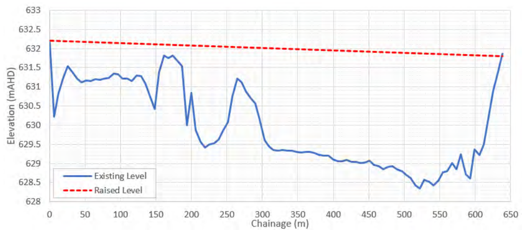
Image 16: Option L04 – long section
